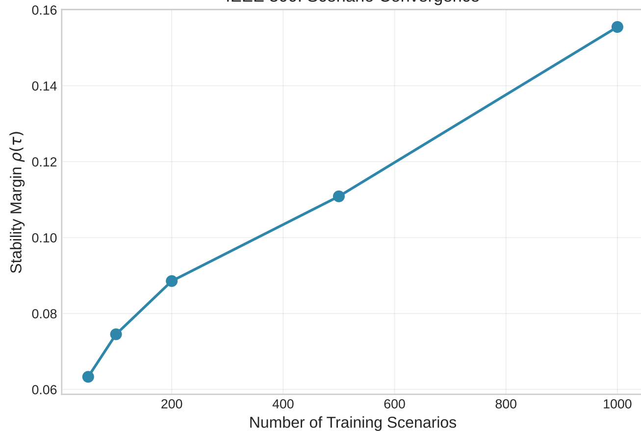
IEEE 300: Scenario Convergence
