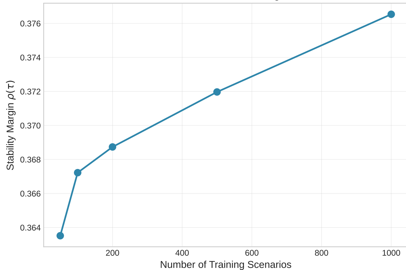
IEEE 57: Scenario Convergence
