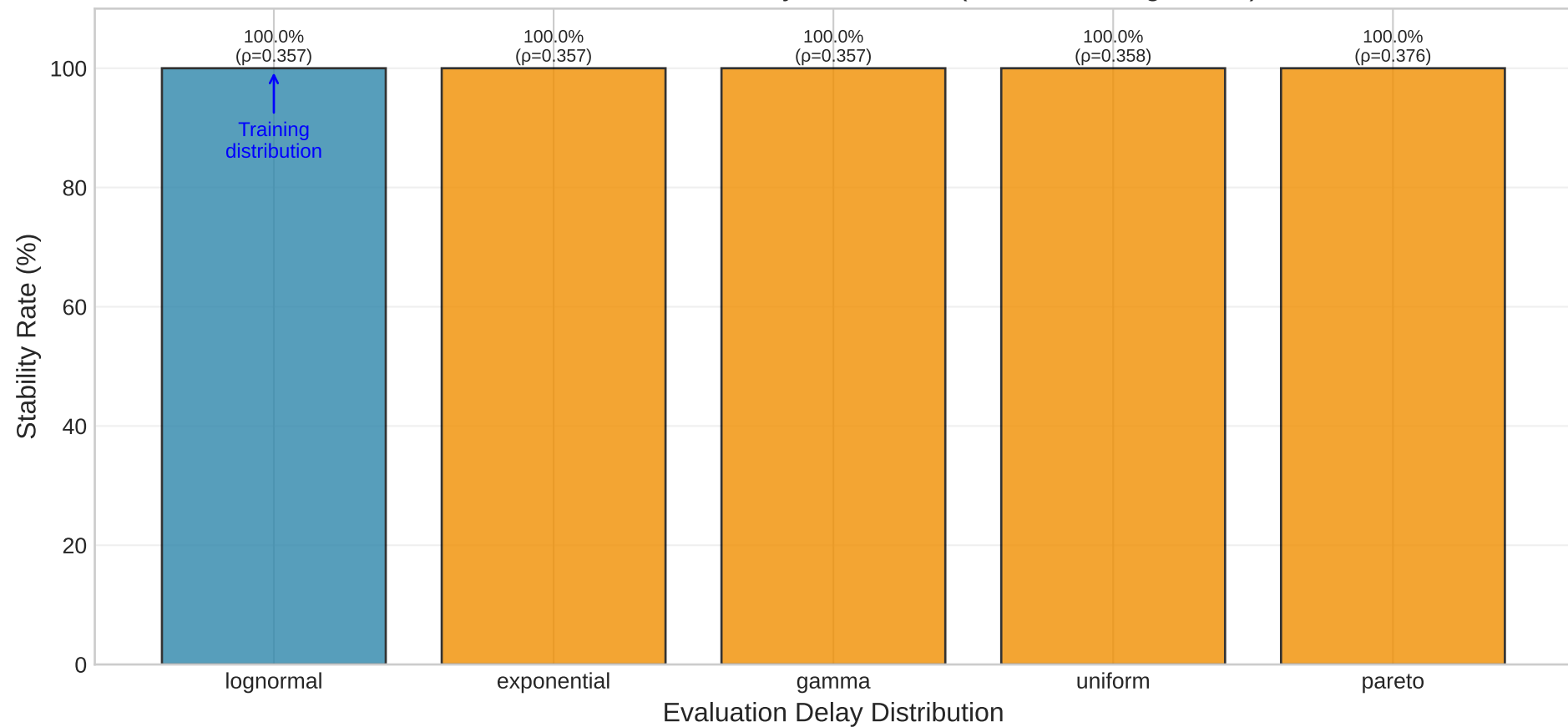
IEEE 14: Robustness to Delay Distribution (Trained on Lognormal)
