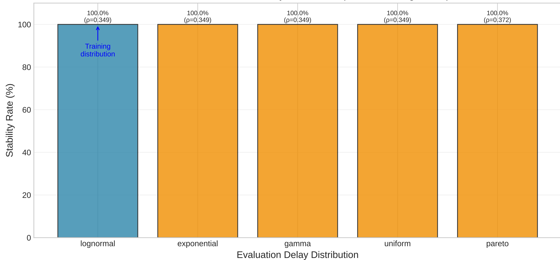
IEEE 30: Robustness to Delay Distribution (Trained on Lognormal)
