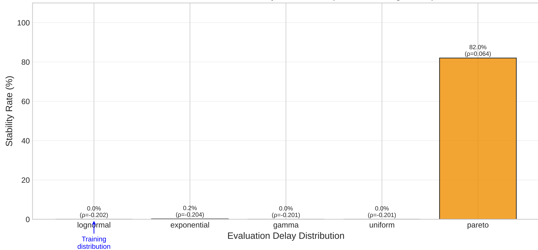
IEEE 300: Robustness to Delay Distribution (Trained on Lognormal)
