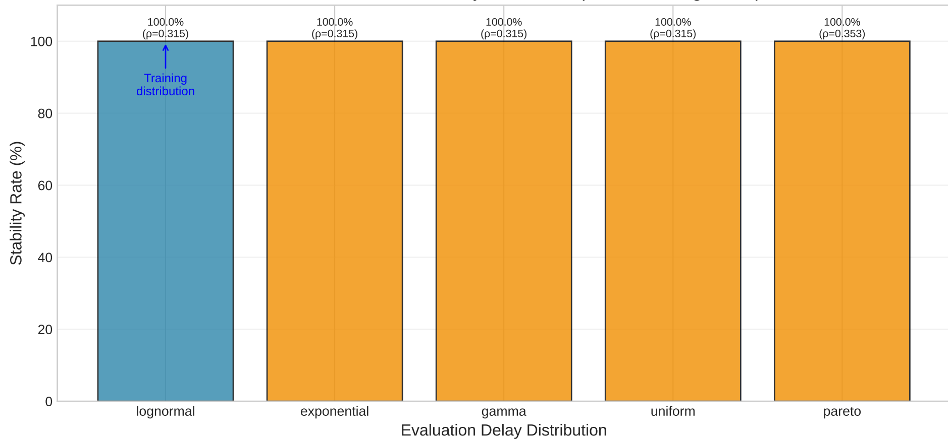
IEEE 39: Robustness to Delay Distribution (Trained on Lognormal)
