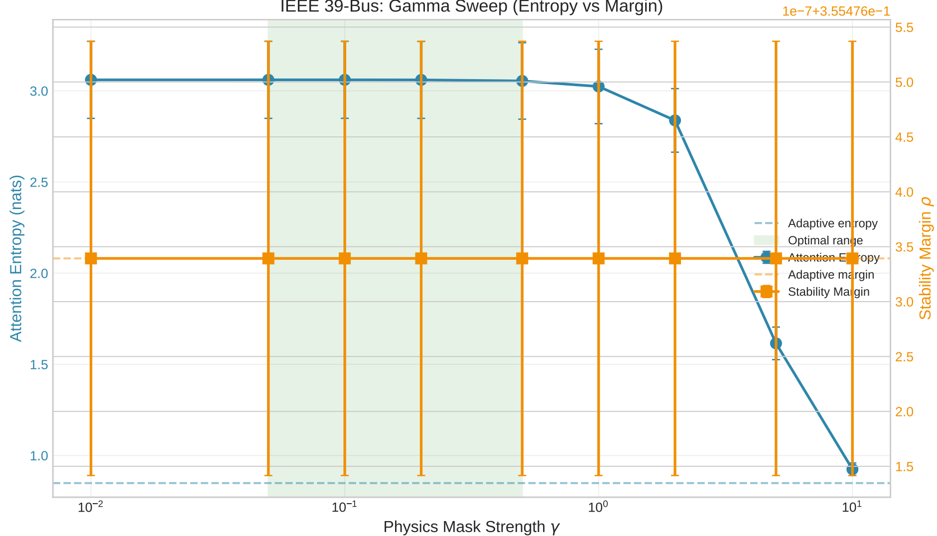
IEEE 39-Bus: Gamma Sweep (Entropy vs Margin)
