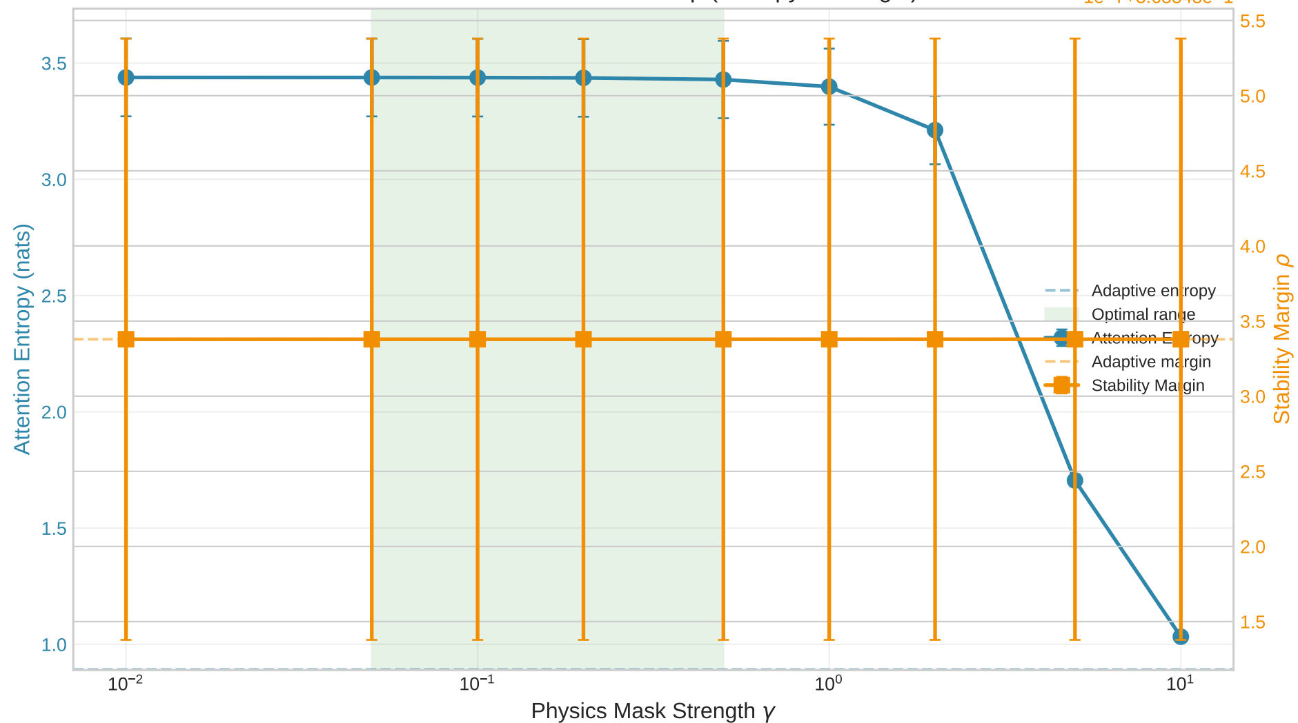
IEEE 57-Bus: Gamma Sweep (Entropy vs Margin)
