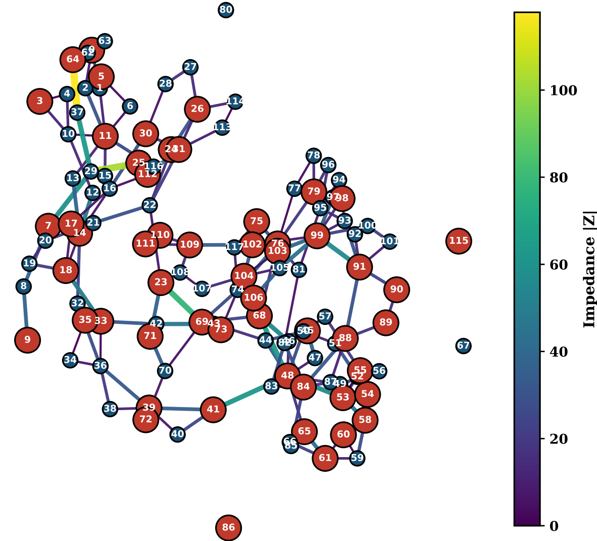
(c) Physical Coupling (edge color = impedance)
