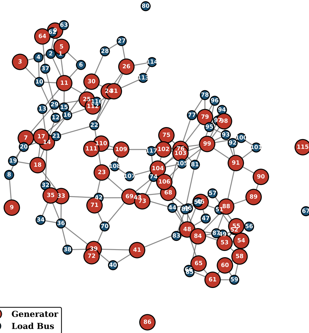
(a) Case-118-Bus Topology (54 generators, 118 buses)
