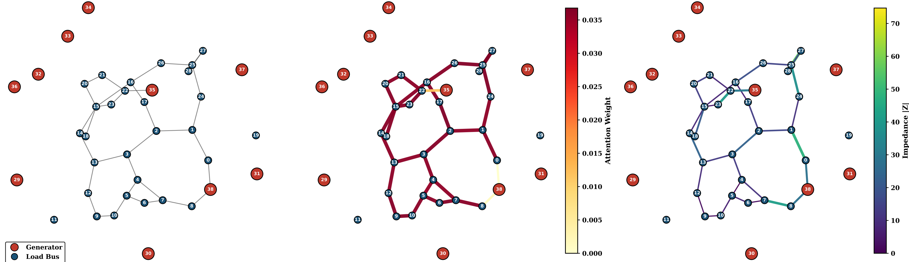
(a) Case-39-Bus Topology (10 generators, 39 buses)
