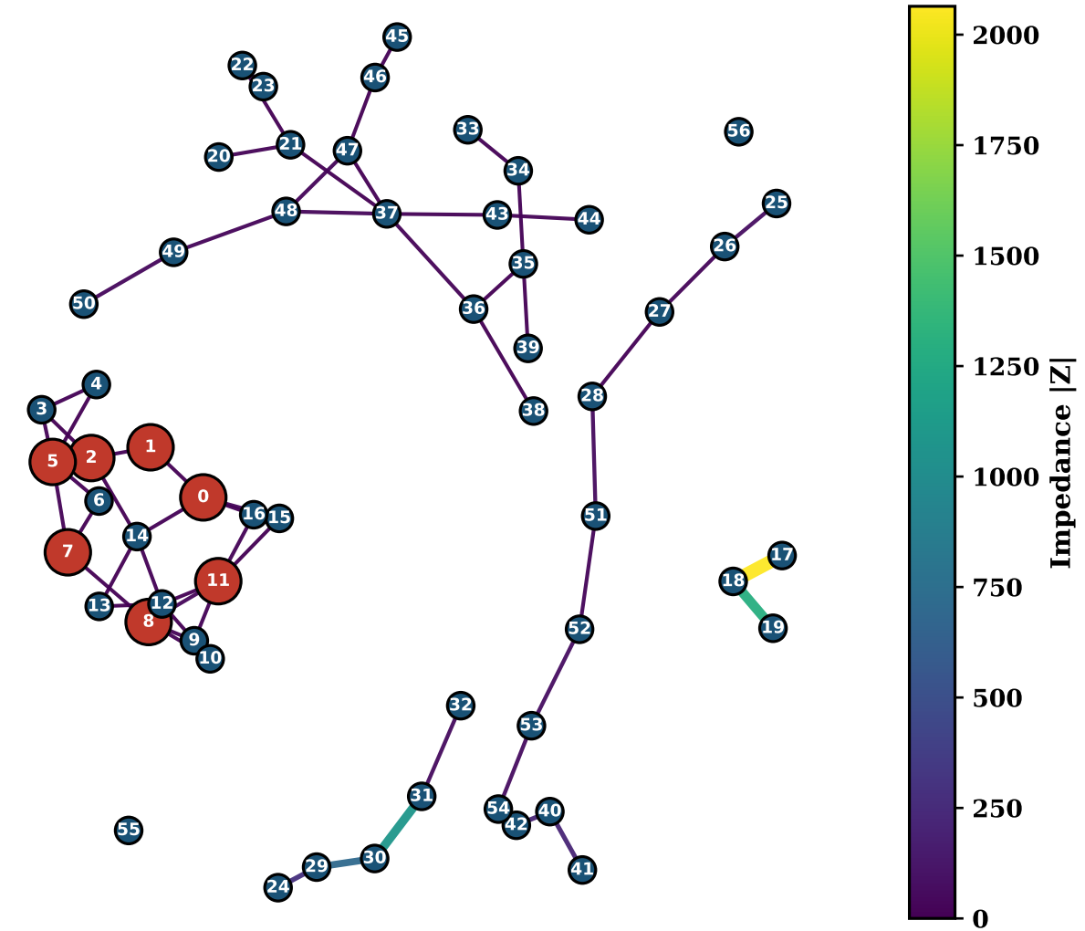
(c) Physical Coupling (edge color = impedance)
