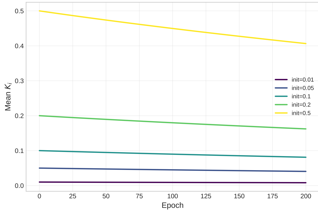
IEEE 14: K Learning Trajectories
