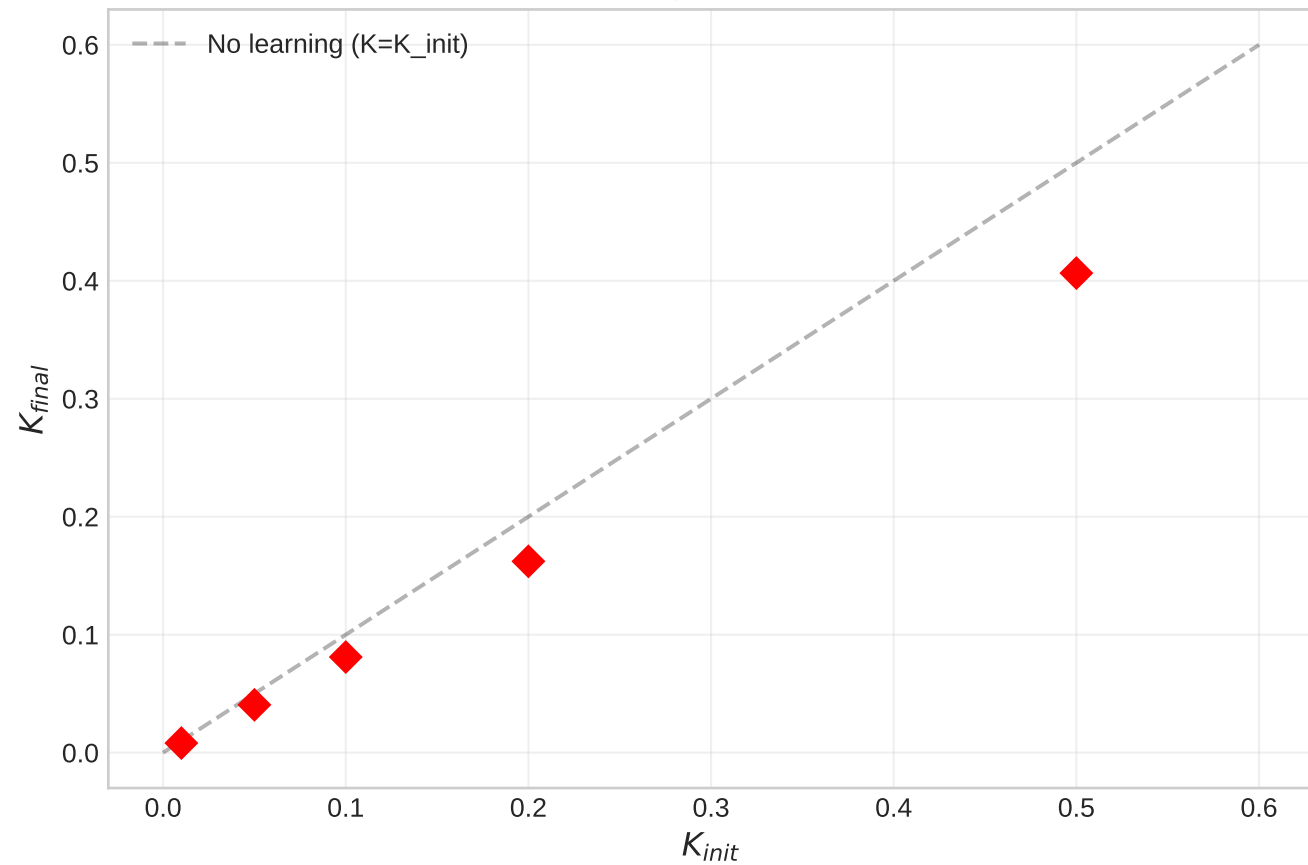
IEEE 14: K Convergence from Different Inits
