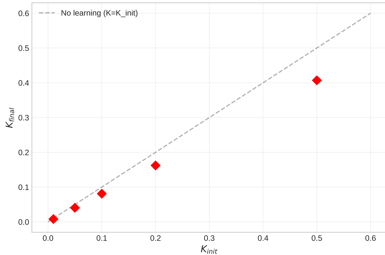
IEEE 30: K Convergence from Different Inits
