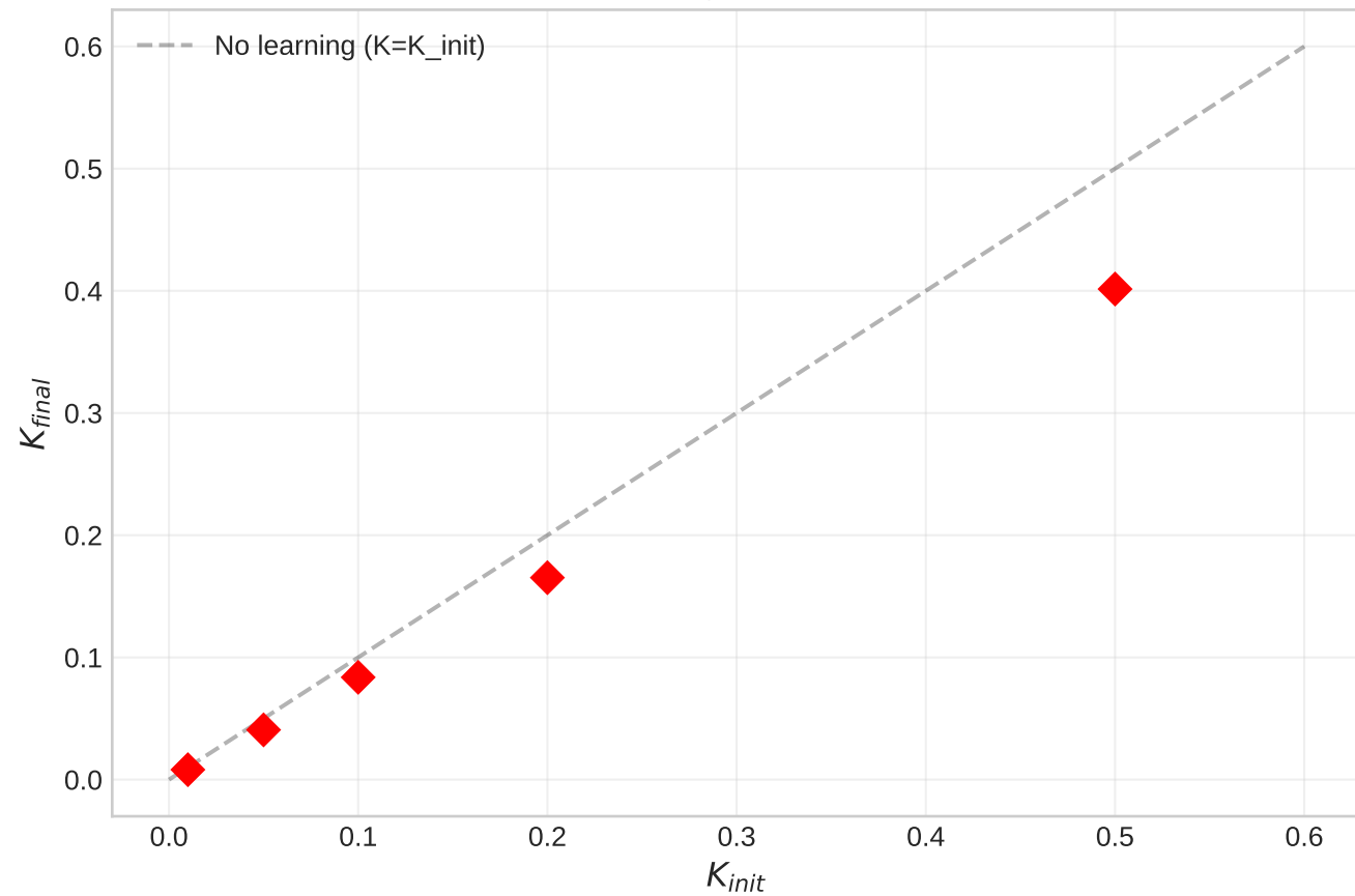
IEEE 300: K Convergence from Different Inits
