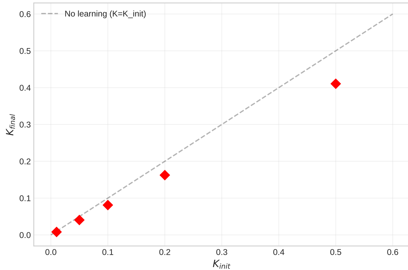
IEEE 39: K Convergence from Different Inits
