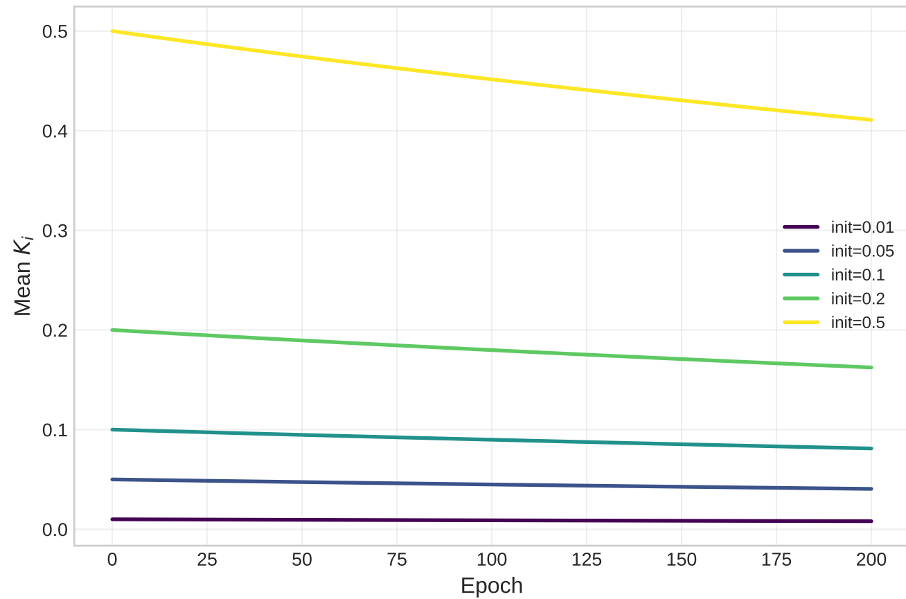
IEEE 39: K Learning Trajectories
