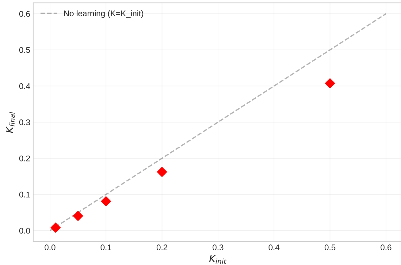
IEEE 57: K Convergence from Different Inits
