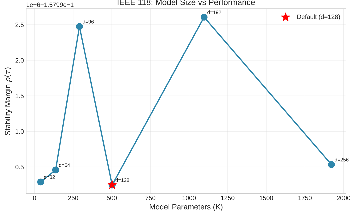
IEEE 118: Model Size vs Performance
