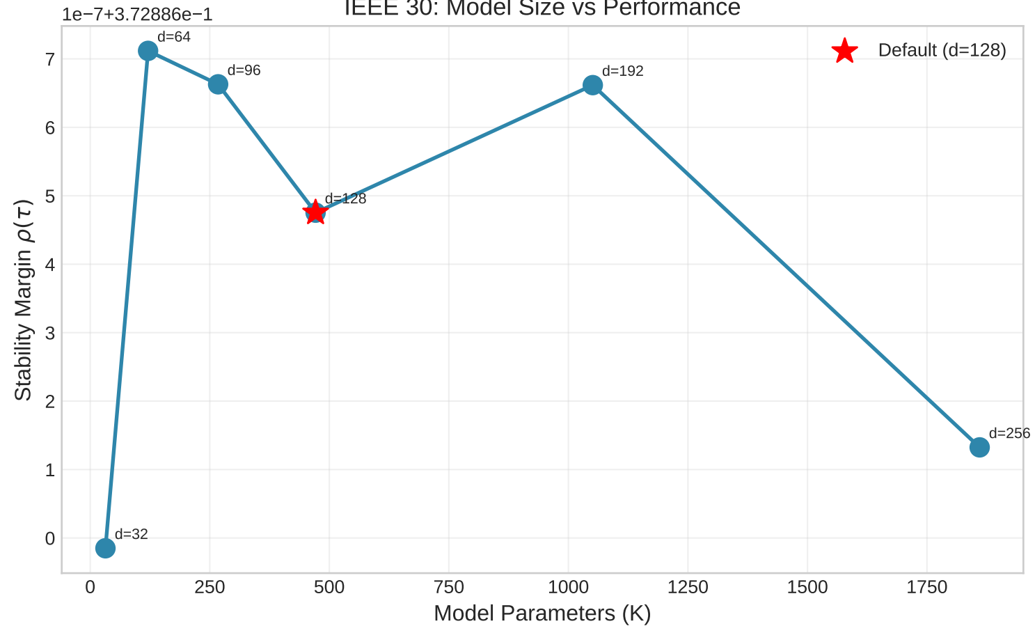
IEEE 30: Model Size vs Performance
