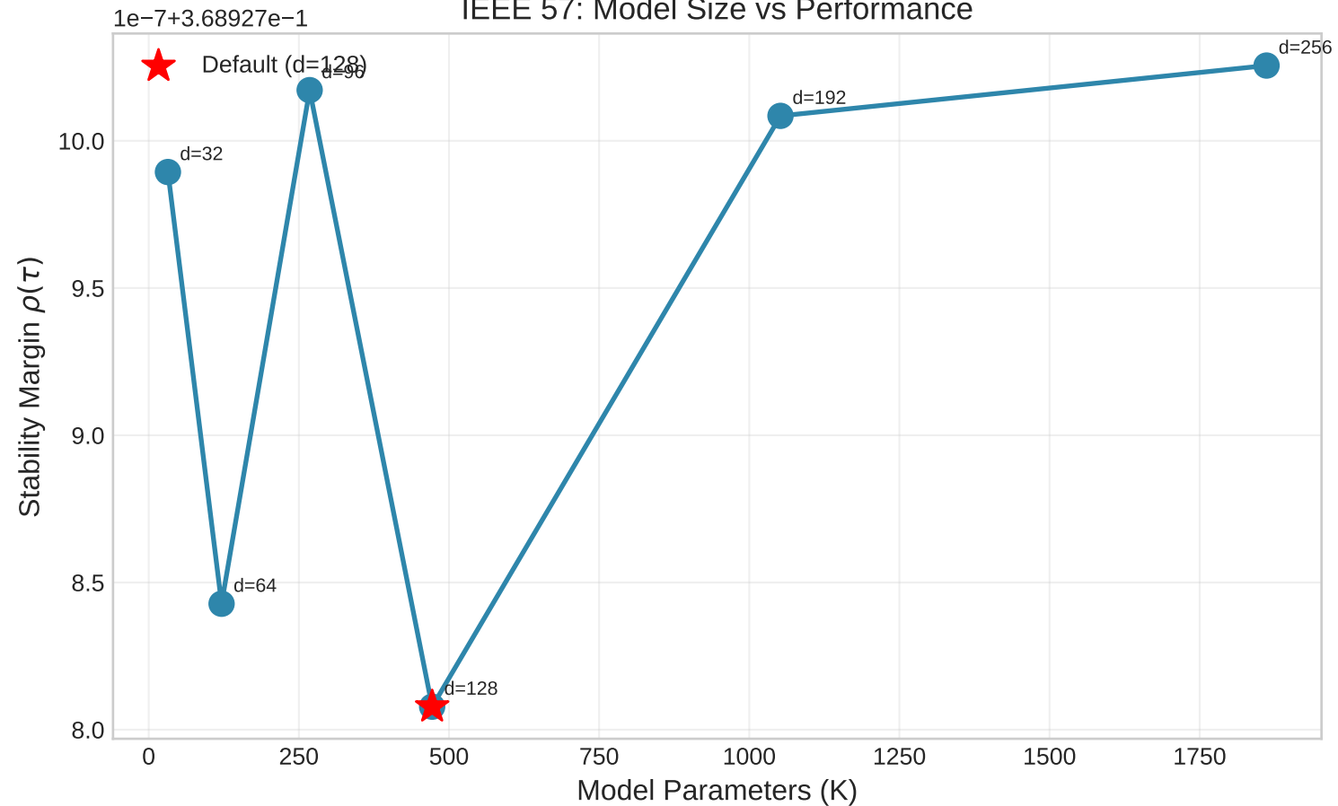
IEEE 57: Model Size vs Performance
