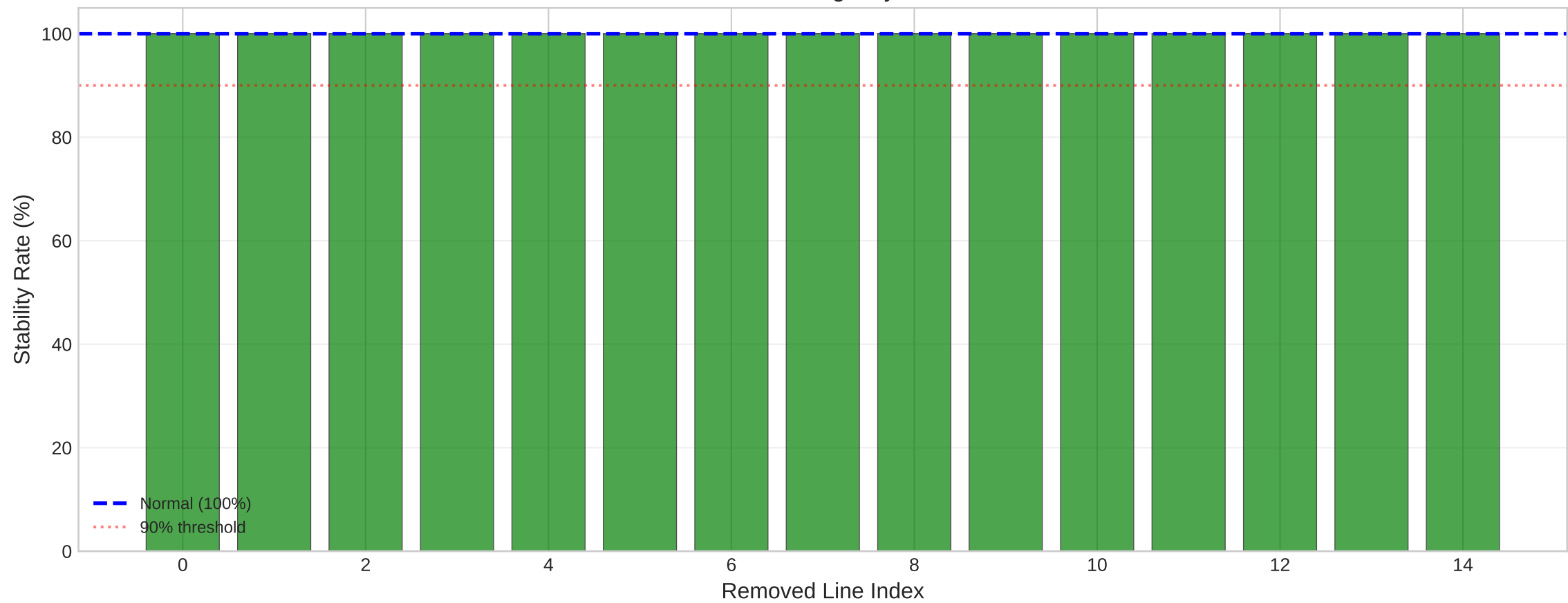
IEEE 14: N-1 Contingency Robustness
