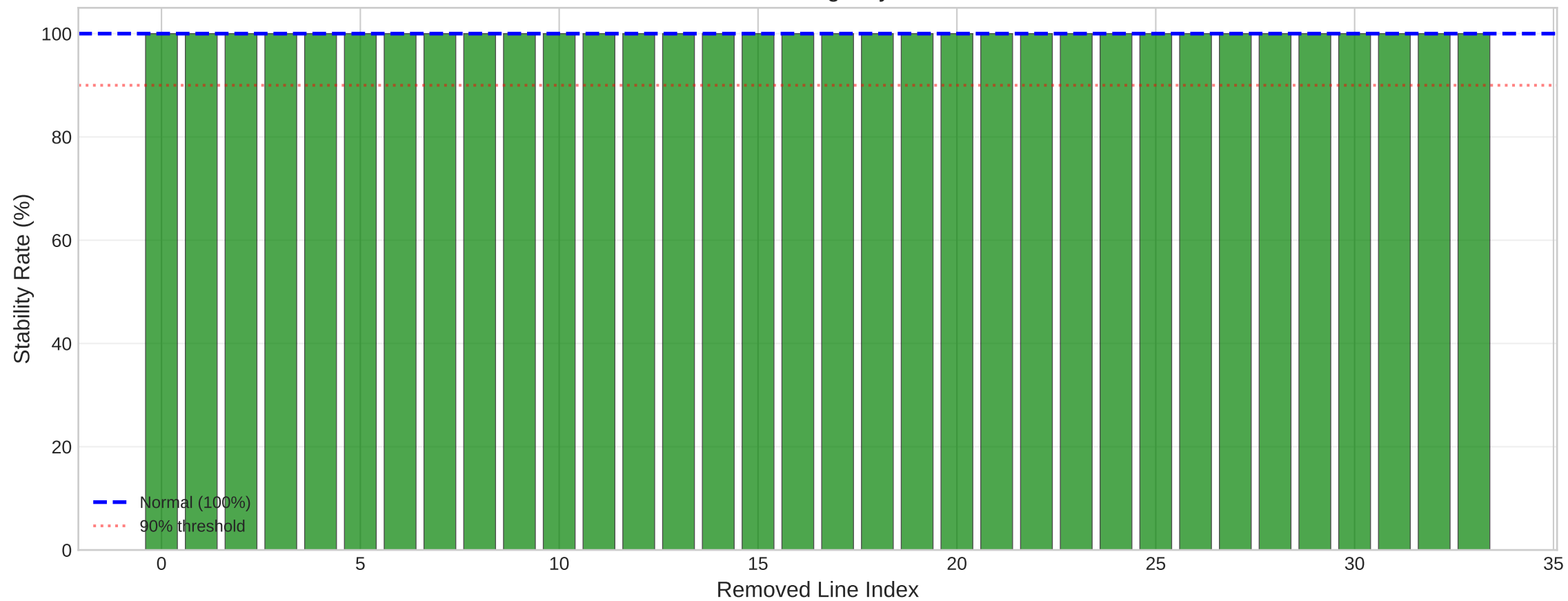
IEEE 30: N-1 Contingency Robustness
