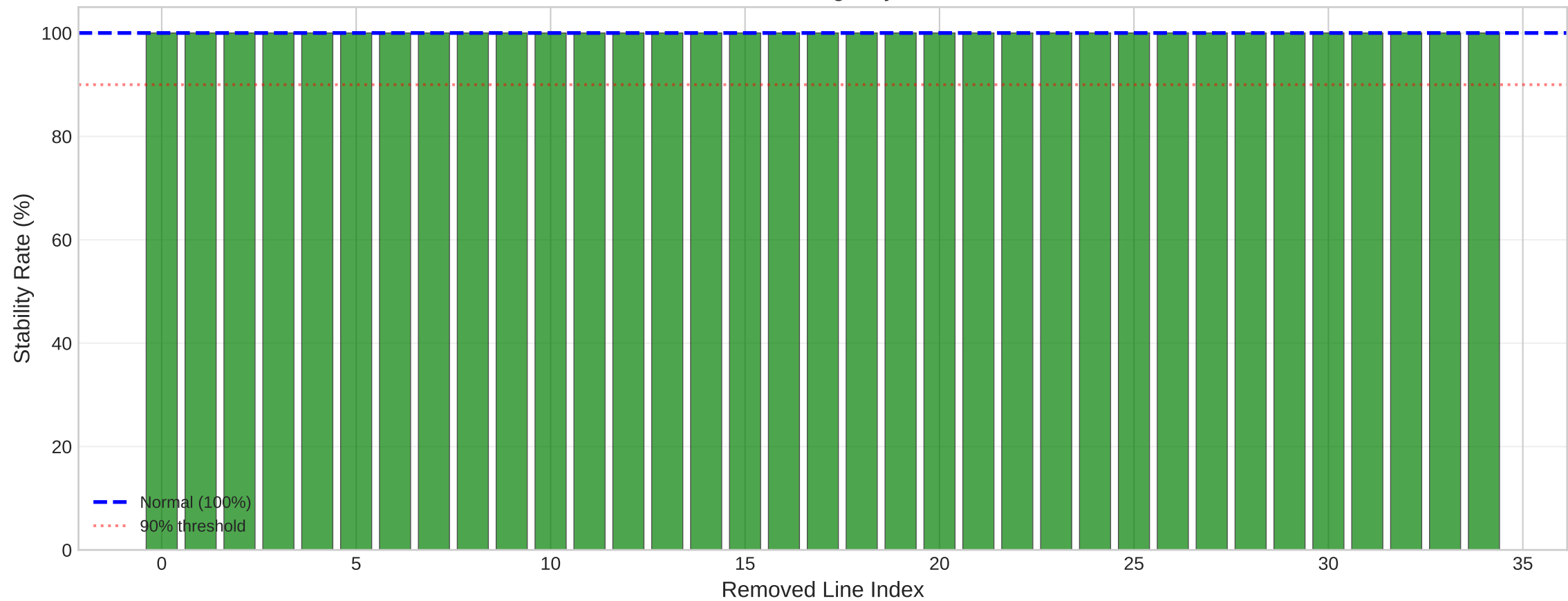
IEEE 39: N-1 Contingency Robustness
