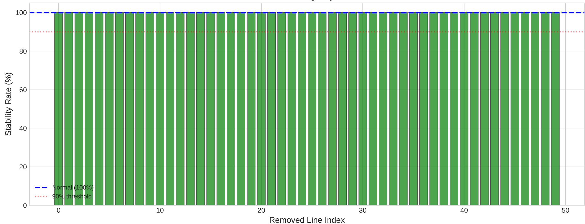
IEEE 57: N-1 Contingency Robustness
