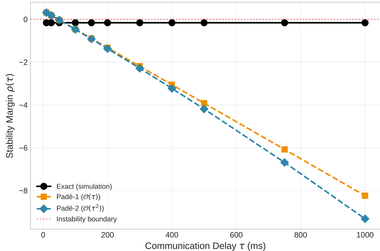
IEEE 118: Padé Approximation Accuracy
