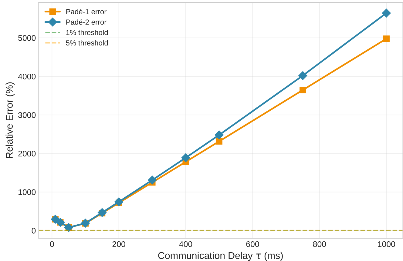
IEEE 118: Approximation Error
