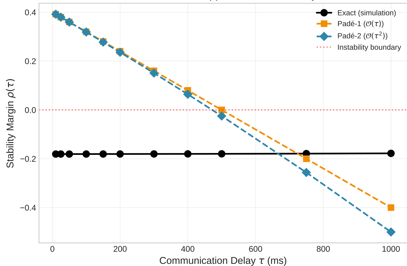
IEEE 14: Padé Approximation Accuracy
