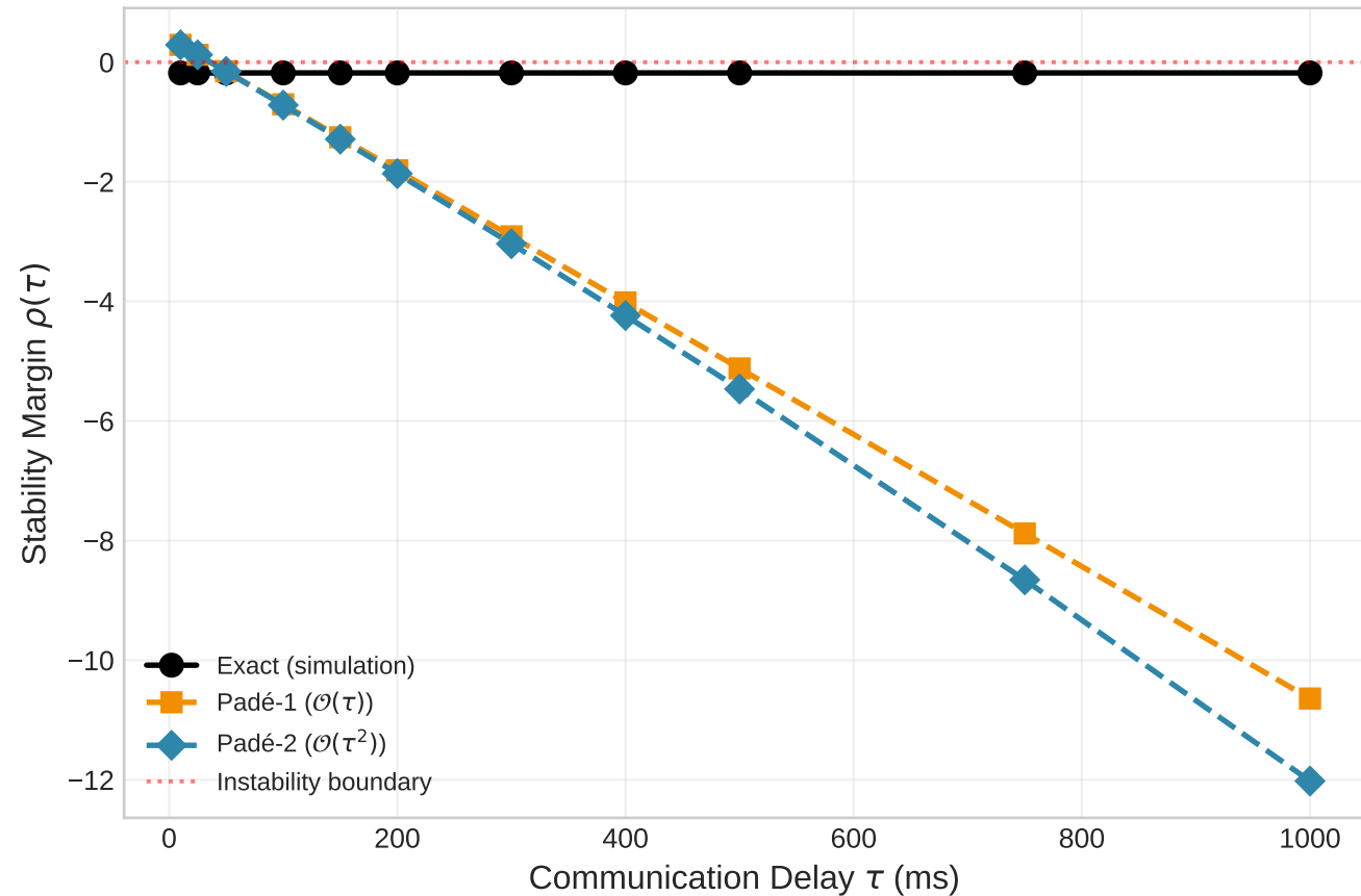
IEEE 300: Padé Approximation Accuracy
