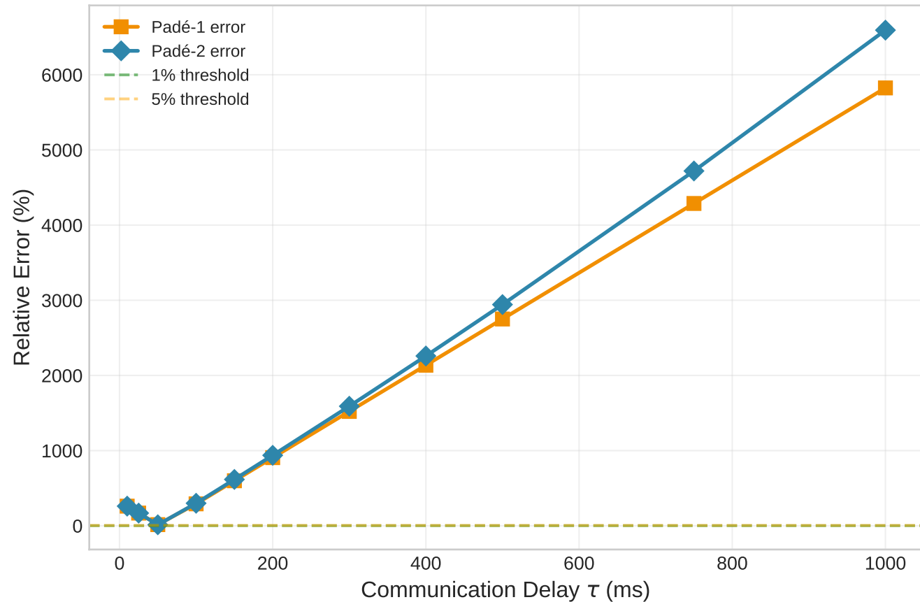
IEEE 300: Approximation Error
