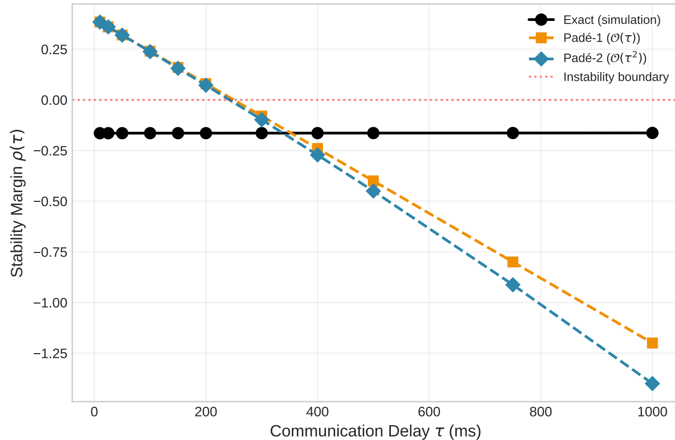
IEEE 39: Padé Approximation Accuracy
