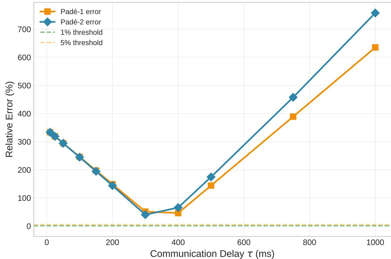
IEEE 39: Approximation Error
