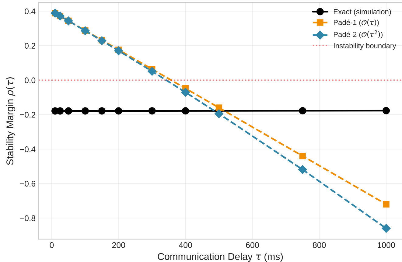
IEEE 57: Padé Approximation Accuracy
