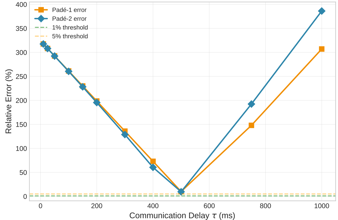
IEEE 57: Approximation Error
