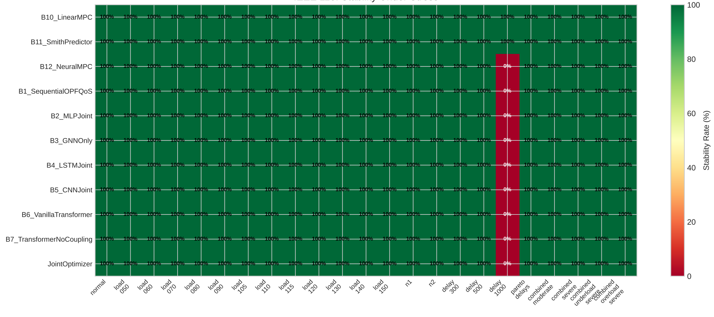
IEEE 118: Stability Under Stress
