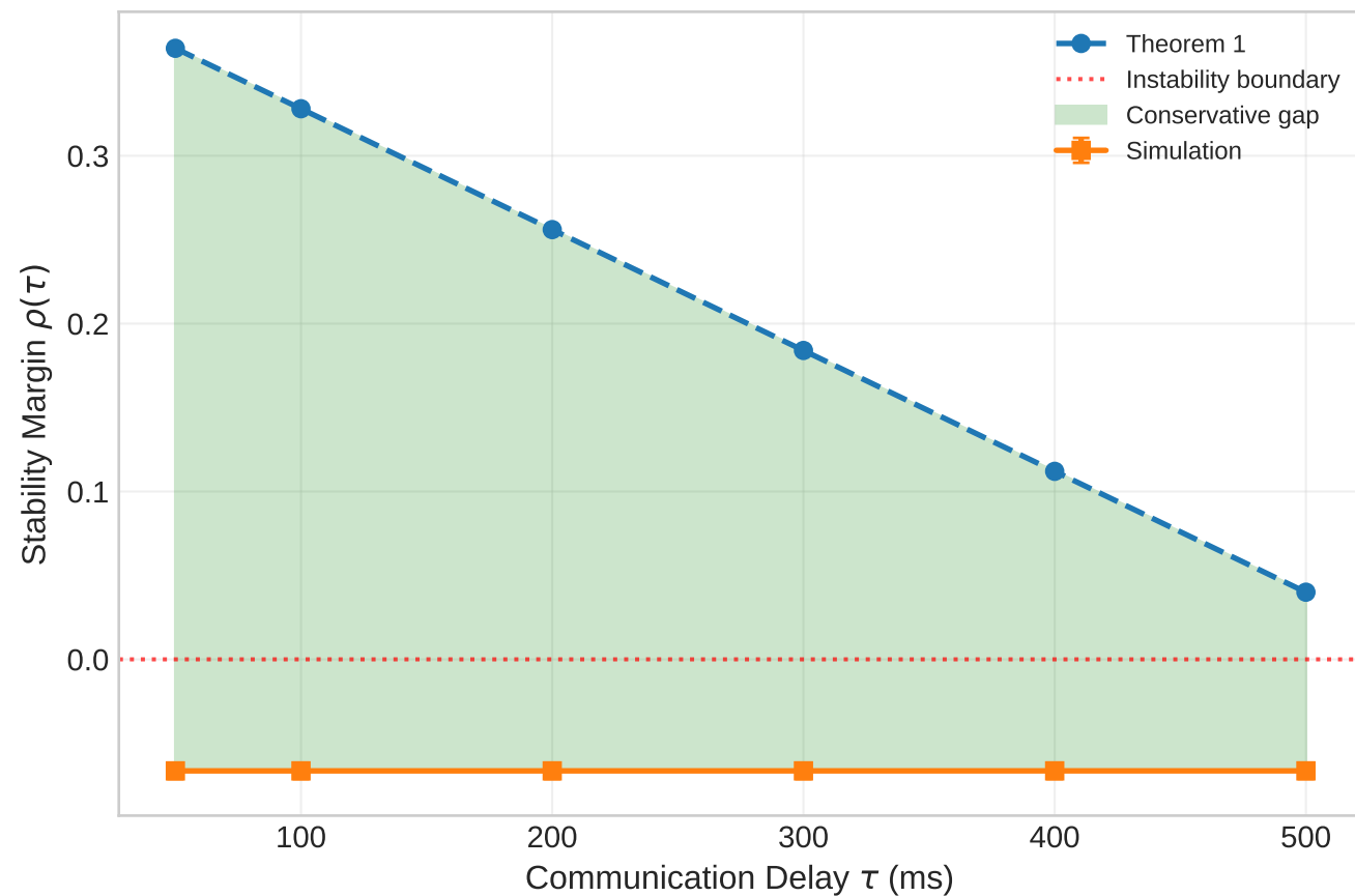
IEEE 118-Bus: Theorem 1 Bound vs Simulation
