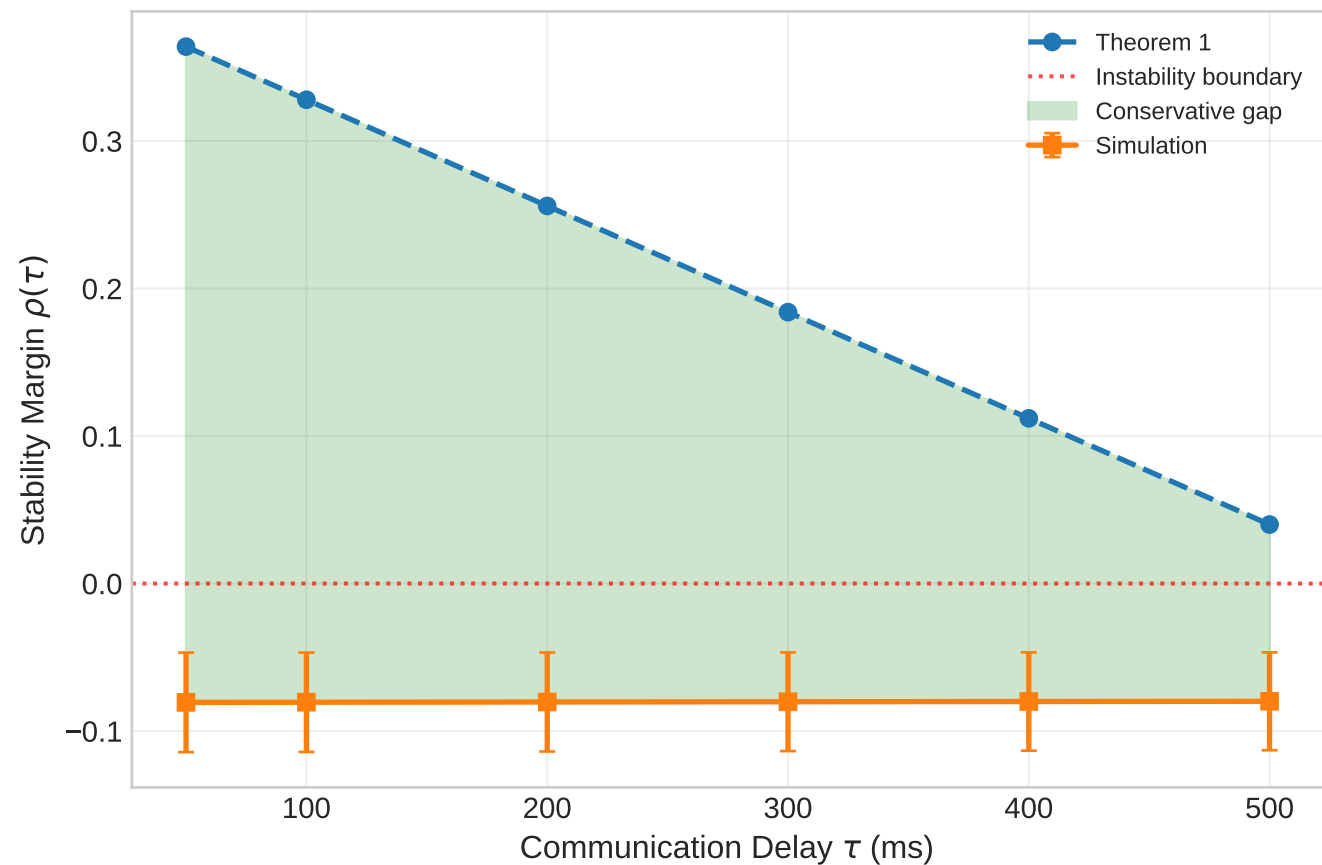
IEEE 14-Bus: Theorem 1 Bound vs Simulation
