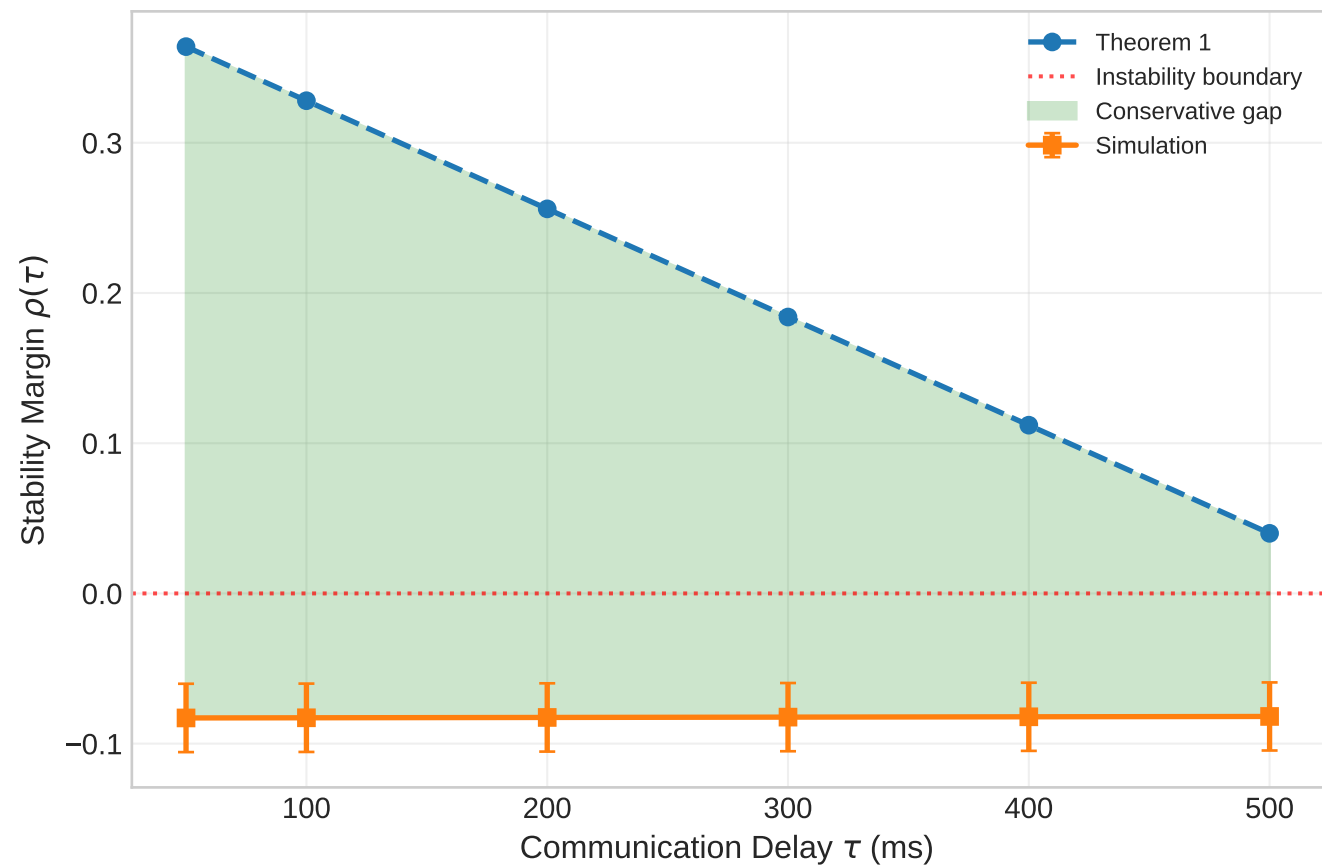
IEEE 30-Bus: Theorem 1 Bound vs Simulation
