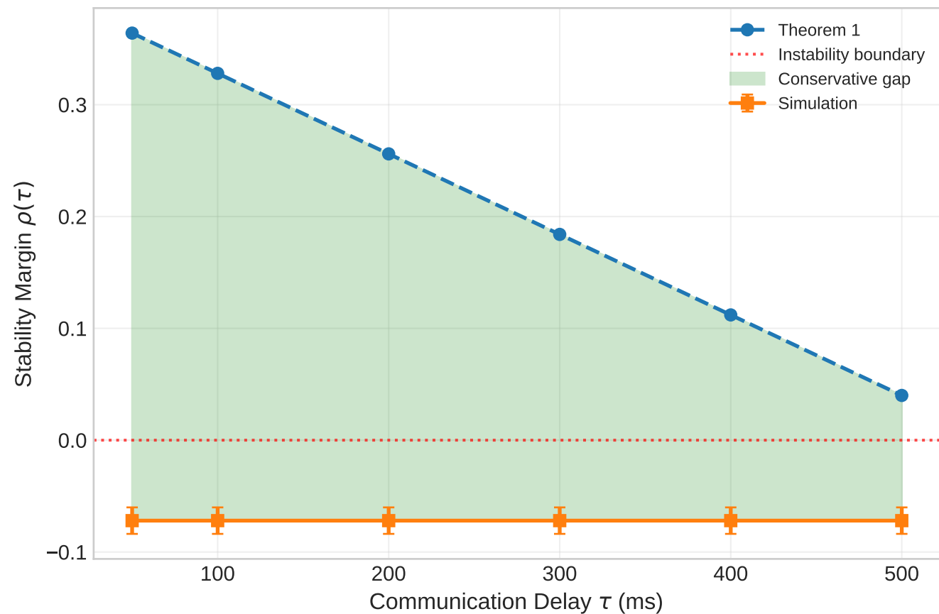
IEEE 300-Bus: Theorem 1 Bound vs Simulation
