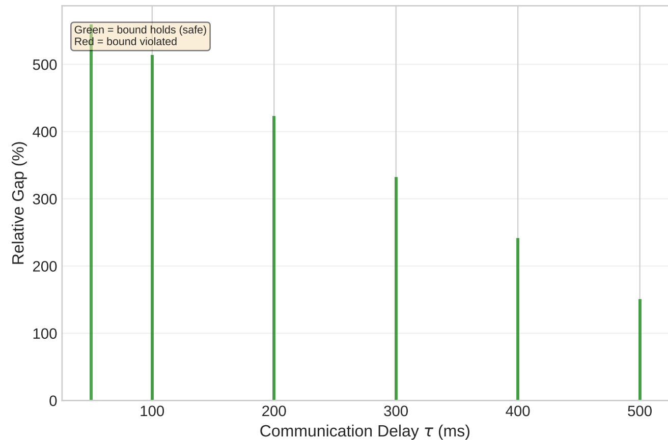
Theorem 1 Conservatism
