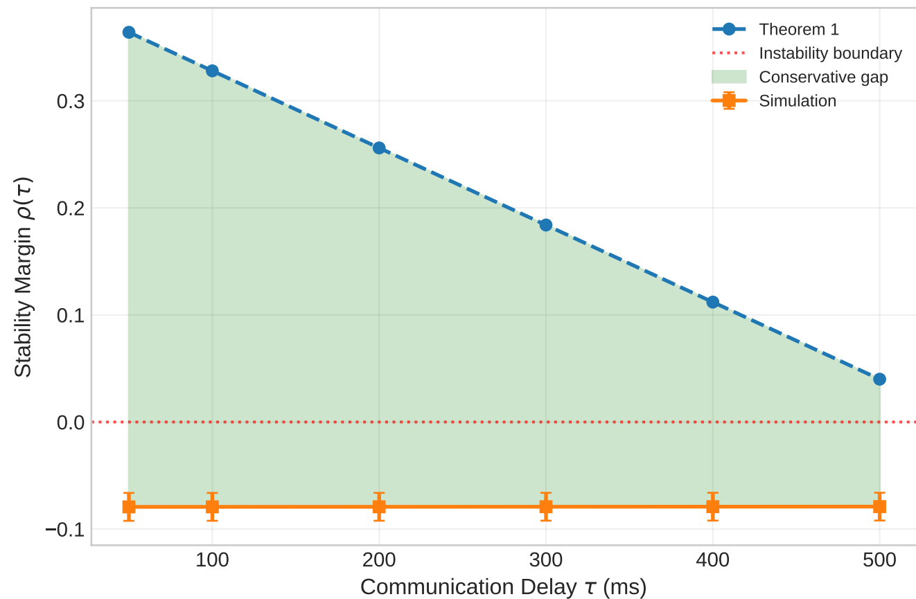
IEEE 39-Bus: Theorem 1 Bound vs Simulation
