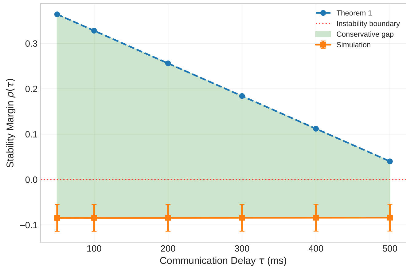
IEEE 57-Bus: Theorem 1 Bound vs Simulation
