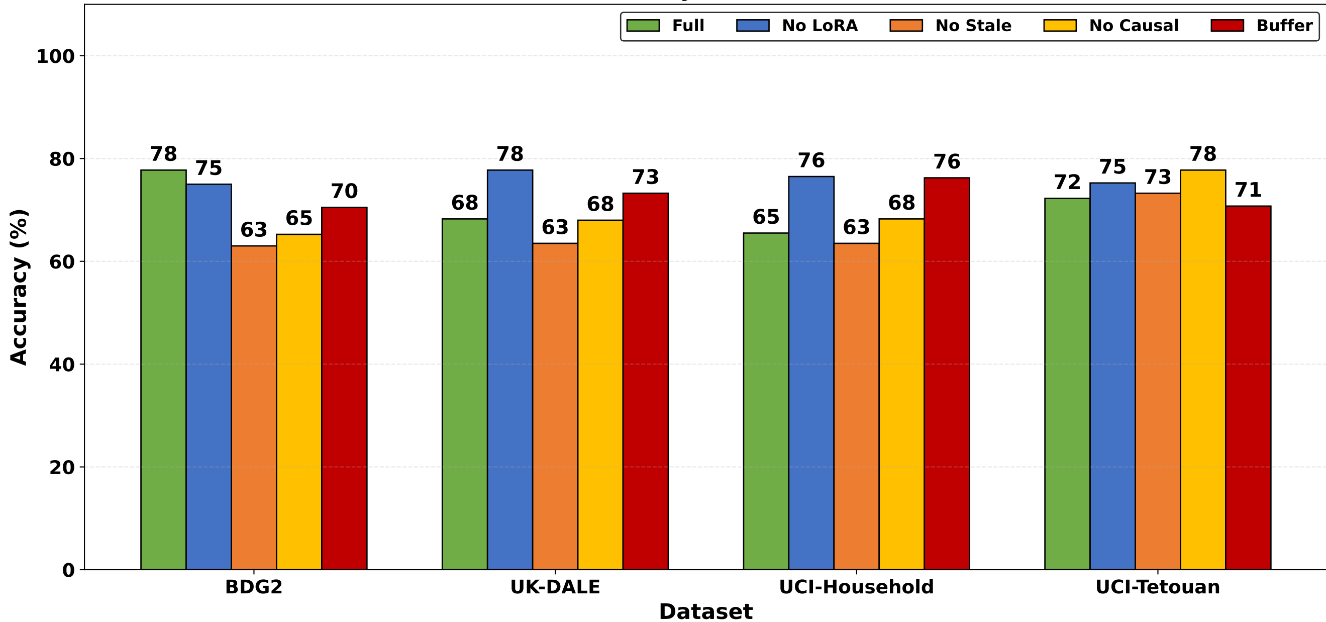
Ablation Study Across Datasets
