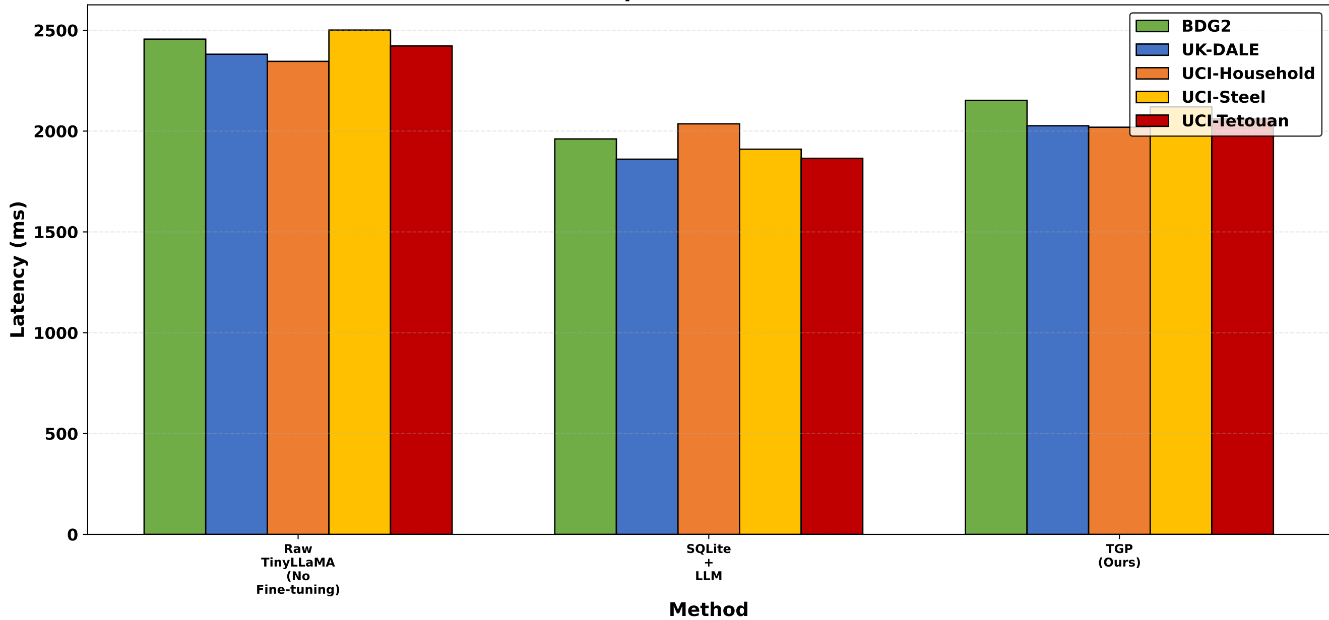
SOTA Comparison Across Datasets
