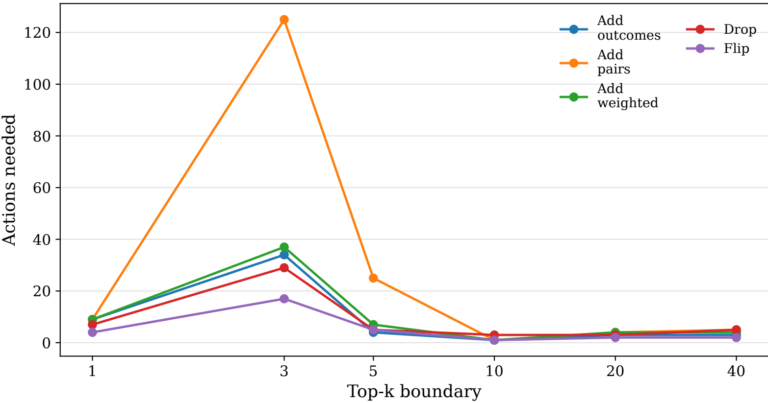
Arena55k: actions needed to change top-k
