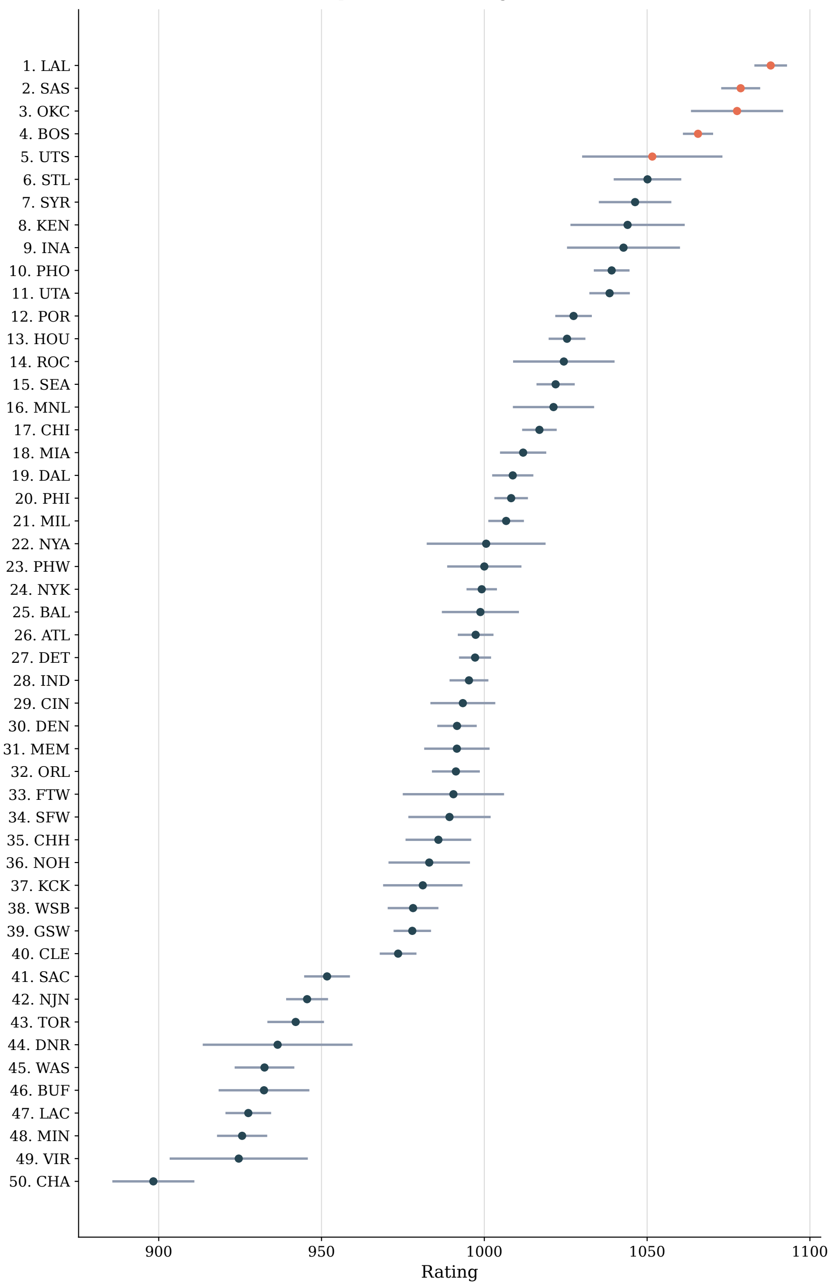
NBA Elo Top-50 Teams ranking with Gao 95% CI
