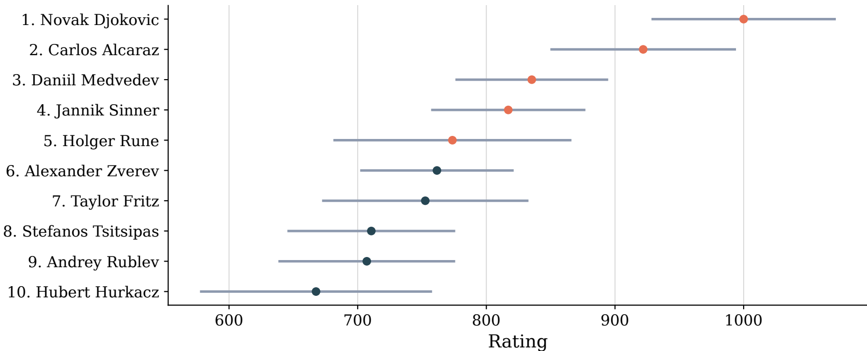
ATP Top-10 Matchups (2020-2024) ranking with Gao 95% CI
