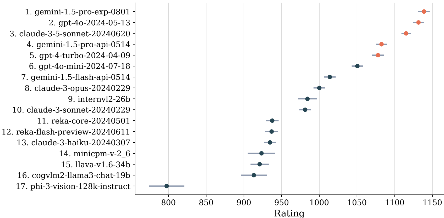
Vision Arena ranking with Gao 95% CI
