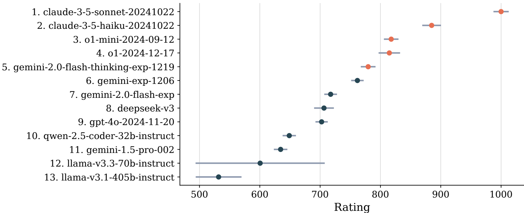
WebDev Arena ranking with Gao 95% CI
