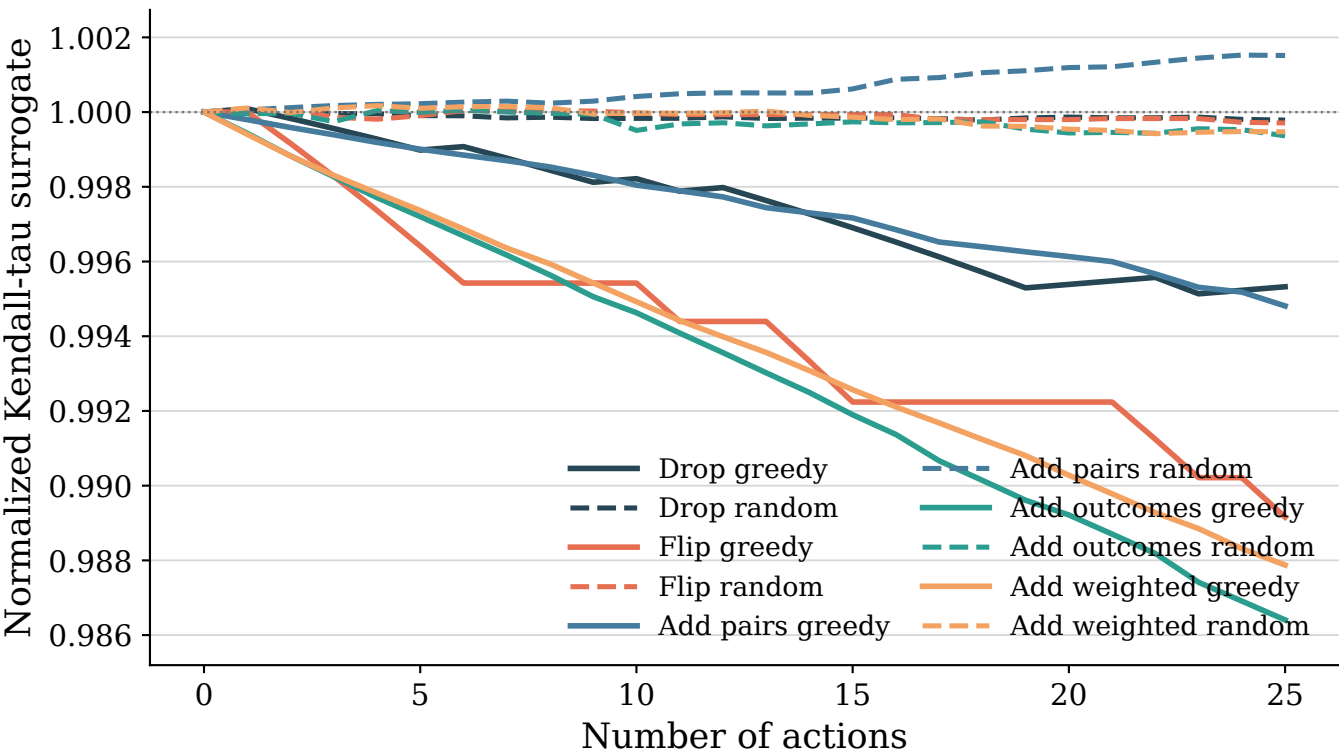
Chatbot Arena 55k: Kendall tau vs actions
