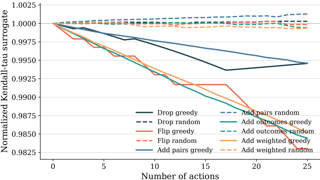
Chatbot Arena LLM Judges: Kendall tau vs actions
