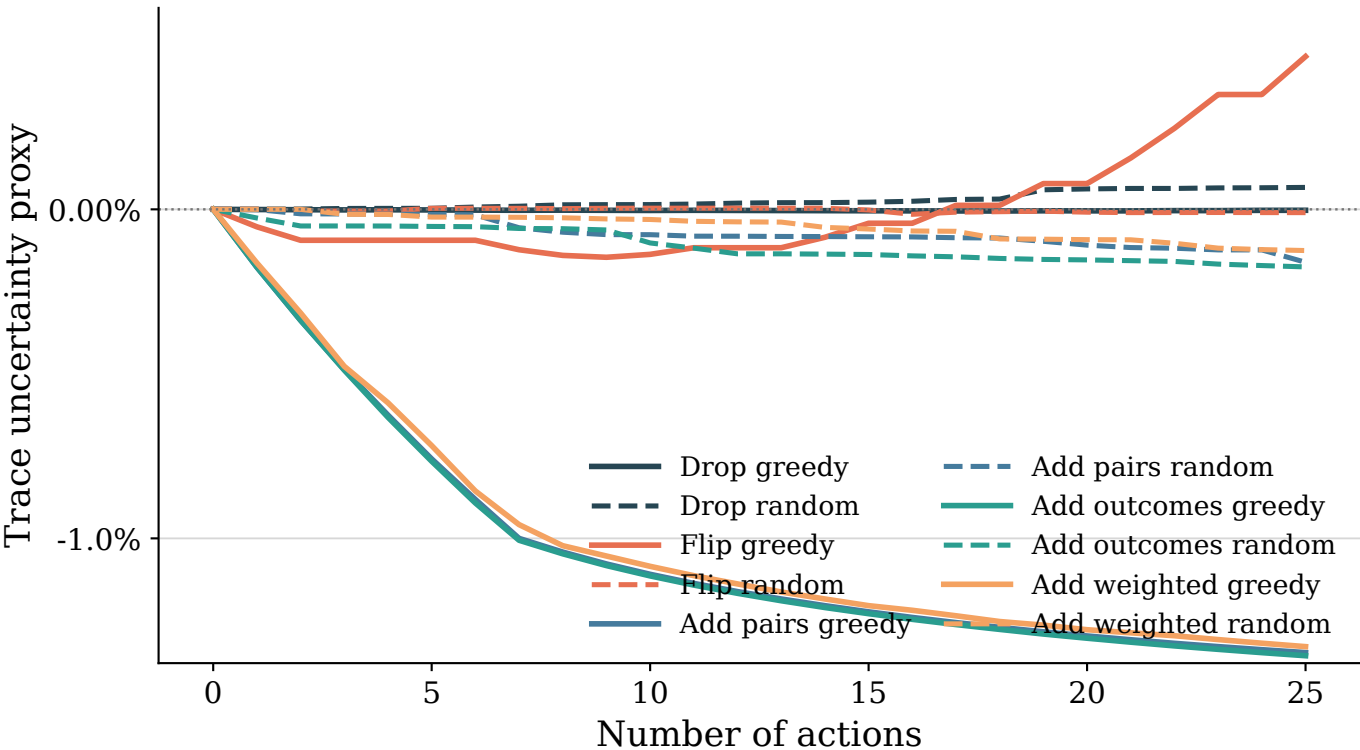
Chatbot Arena LLM Judges: trace uncertainty proxy vs actions
