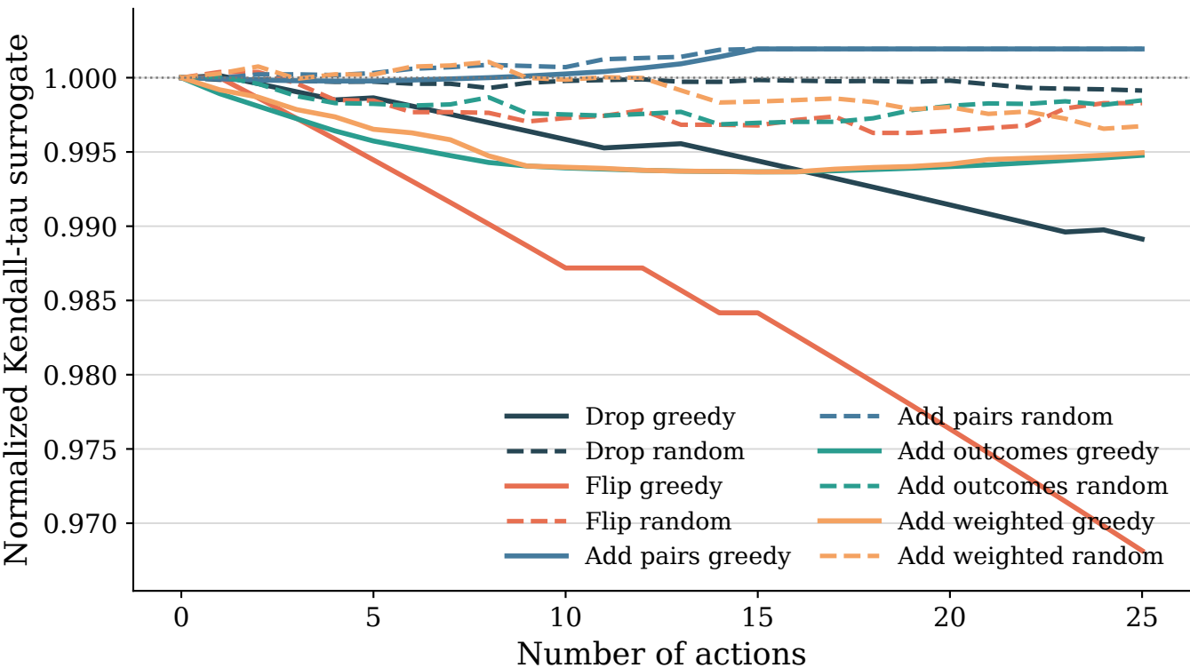
MT-Bench Human Judgments: Kendall tau vs actions
