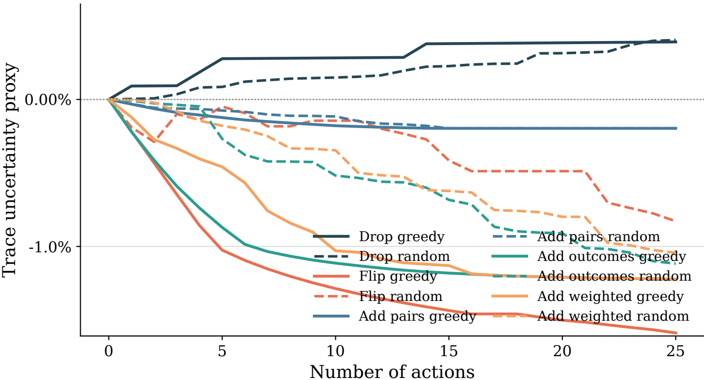
MT-Bench Human Judgments: trace uncertainty proxy vs actions
