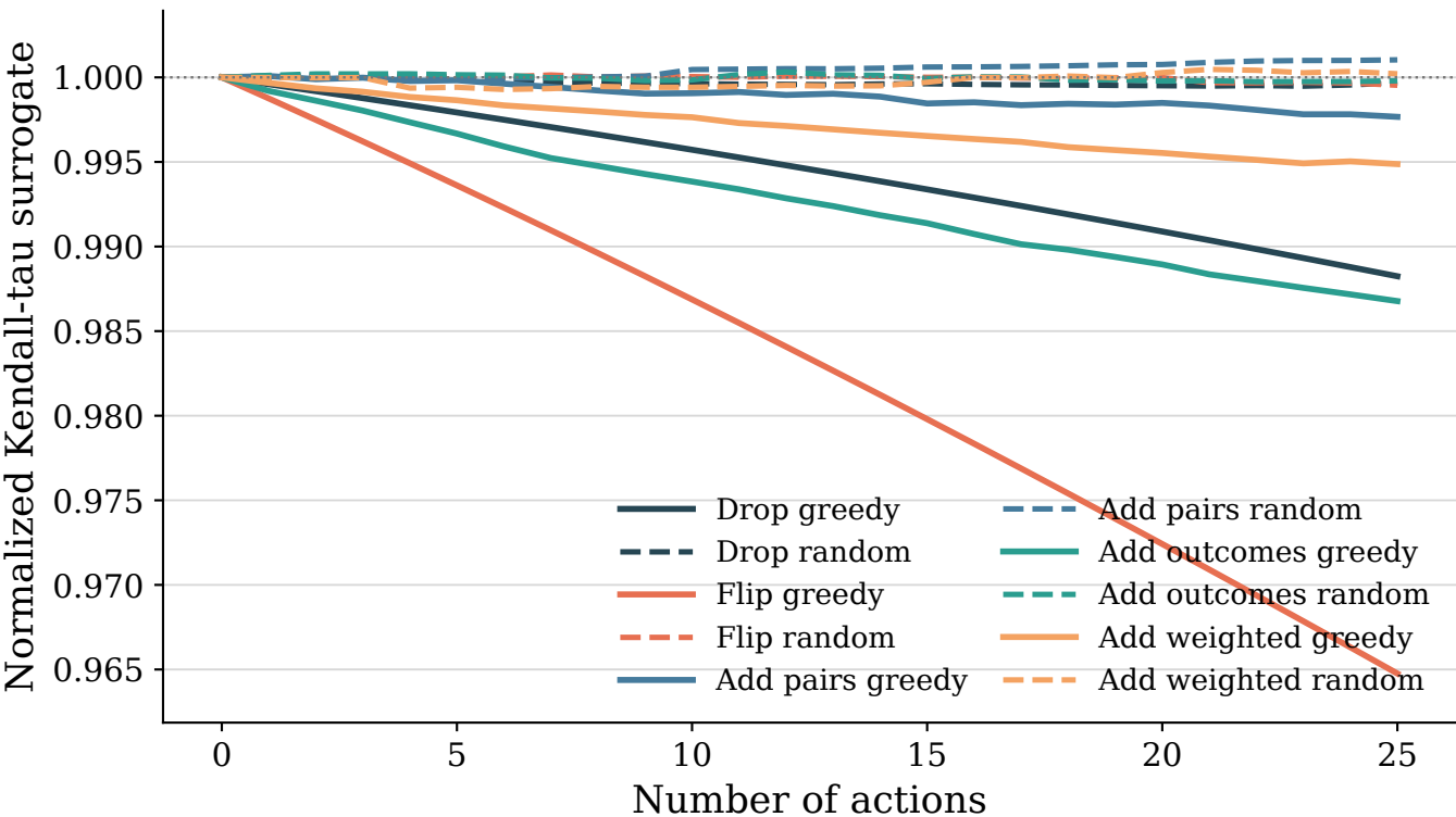
NBA Elo Top-50 Teams: Kendall tau vs actions
