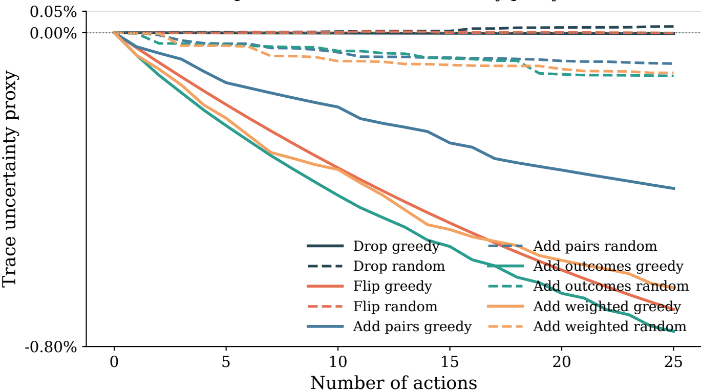
NBA Elo Top-50 Teams: trace uncertainty proxy vs actions
