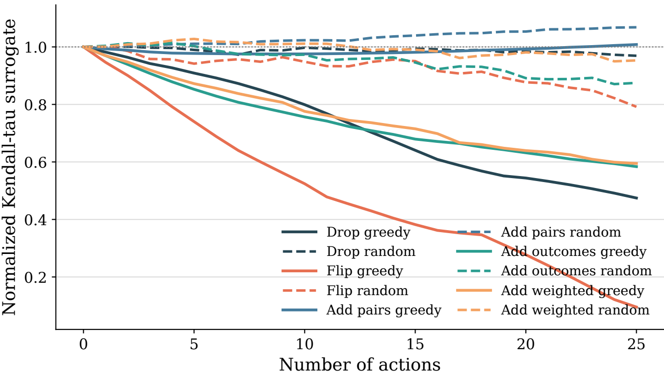
ATP Top-10 Matchups (2020-2024): Kendall tau vs actions
